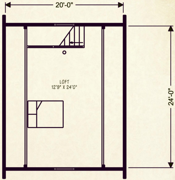
LOFT PLAN 306 SQ. FT.
