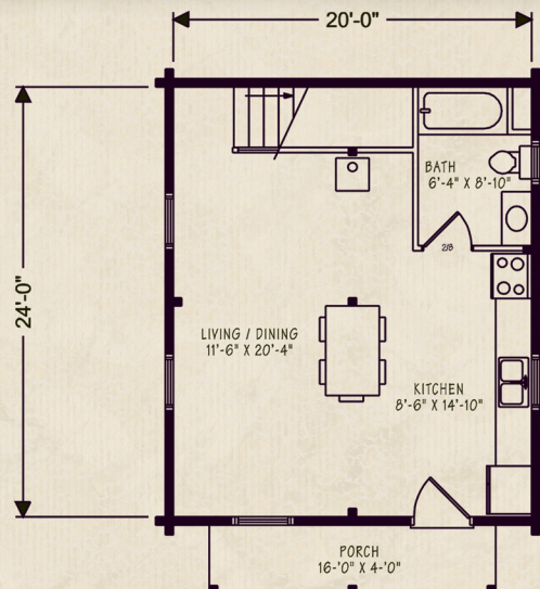
FLOOR PLAN 480 SQ. FT.
