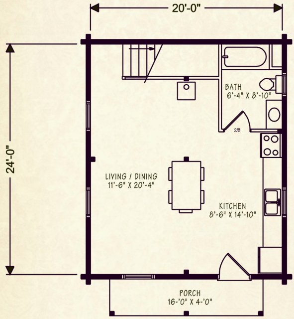
FLOOR PLAN 480 SQ. FT.
