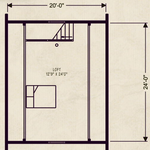
LOFT PLAN 306 SQ. FT.
